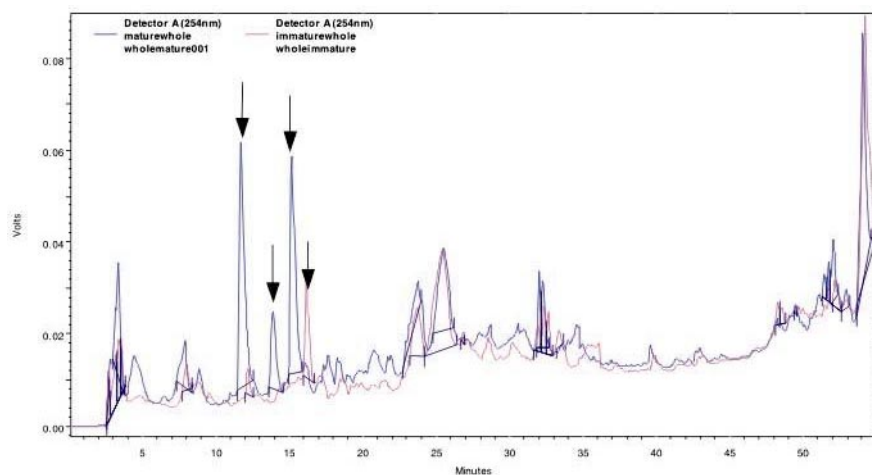
Figure 2. Comparative HPLC profiles of mature and immature tubers of Ipomoea mauritiana (Vidari).
