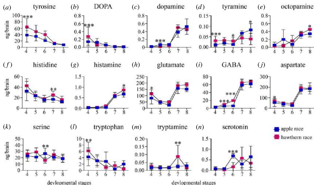
Figure 3. Quantification of biogenic amines and their precursors from the onset of adult brain development (stage 4) all the way up to sexually mature fly (stage 8) as defined in figure 1 ( a–n ). Line graph of neurochemical titres for both host races at different developmental stages with 4–15 n_{\text{samples}} per stage, containing a pool of five brains in each sample. Symbols represent mean with s.e.: ( a ) tyrosine; ( b ) DOPA; ( c ) dopamine; ( d ) tyramine; ( e ) octopamine; ( f ) histidine; ( g ) histamine; ( h ) glutamate; ( i ) GABA; ( j ) aspartate; ( k ) serine; ( l ) tryptophan; ( m ) tryptamine; and ( n ) serotonin. Asterisks above indicate differences between host races at the equivalent stage of brain development. p -values represented are less than 0.05 *, less than 0.01 ** and less than 0.001 ***, linear mixed effect model, followed by Tukey's HSD correction for multiple comparisons.
