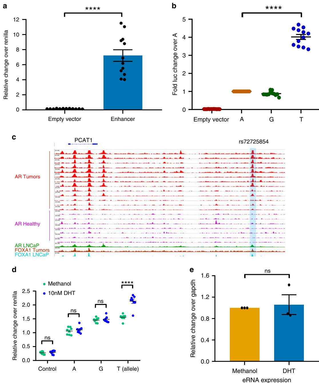
Fig. 2 Risk allele sensitizes the enhancer to androgens. a The graph depicts relative luciferase activity over Renilla for the empty plasmid and the plasmid harboring the rs72725854 enhancer region in LNCaP cells. b The graph depicts the fold change in reporter activity of empty plasmid, “A” and “T” allele over “A” allele in LNCaP cells. Error bars denote SEM from multiple biological replicates ( n > 3 ) in a and b . c UCSC genome browser snapshot around the rs72725854 region with ChIP-seq tracks for AR in tumors, healthy individuals and LNCaP cells and, FOXA1 in tumors and LNCaP cells. d The graph depicts the relative change over Renilla for the empty plasmid and plasmids harboring the different alleles “A”, “G”, and “T” of rs72725854 enhancer in LNCaP cells grown in charcoal stripped media for three days including the treatment with methanol or 10 nM DHT for 16 h. Error bars denote SEM from multiple biological replicates ( n > 3 ). e q-RT PCR analysis showing eRNA expression at rs72725854-harboring enhancer upon 10 nM DHT treatment for 16 h in LNCaP cells. Error bars denote SEM from three biological replicates. p -values were calculated by Student’s two-tailed unpaired t -test in a , b , d , and e ****p < 0.0001 , ^{ns}p > 0.05 . Source data are provided as a Source Data file.
