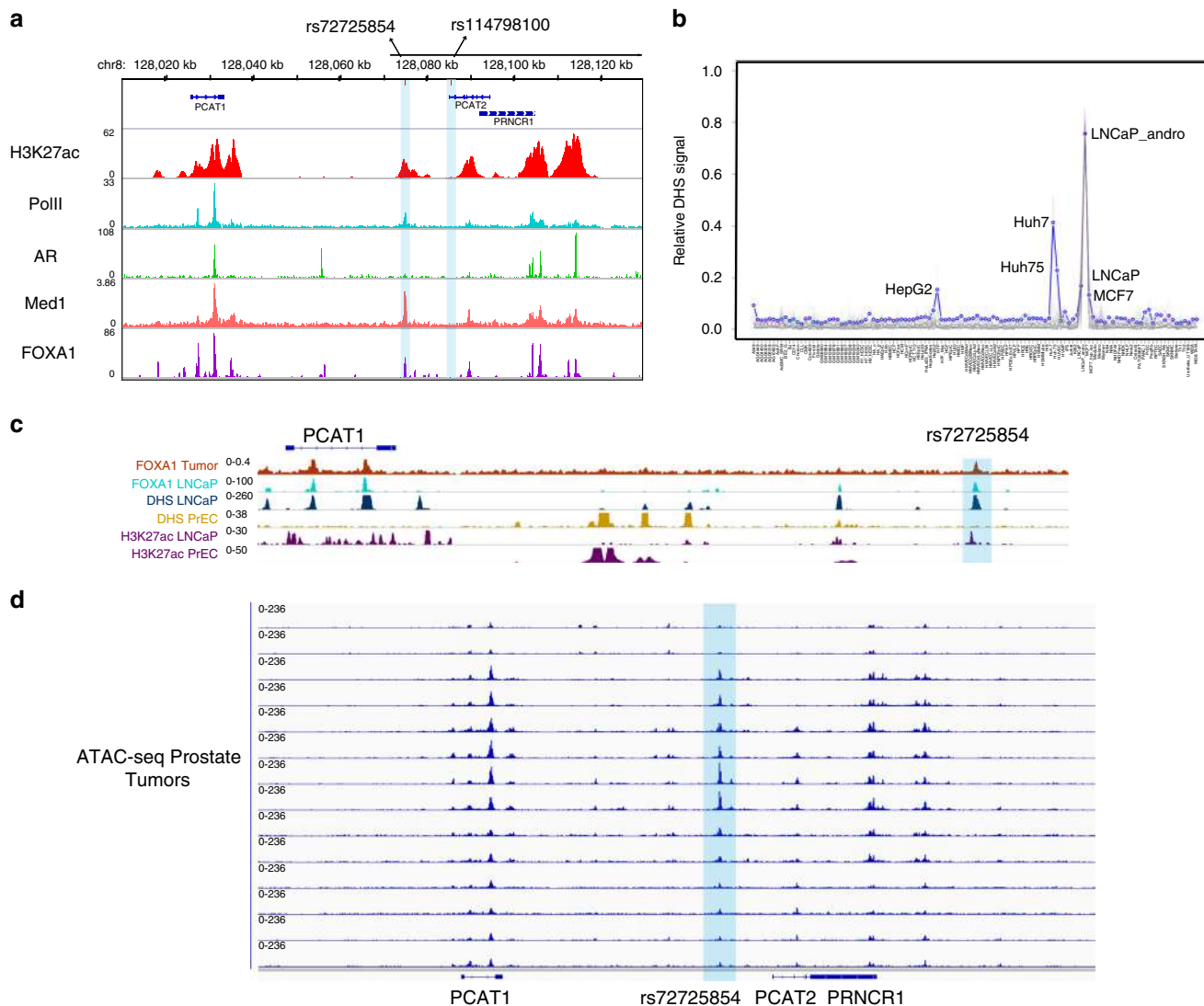
Fig. 1 rs72725854 lies in a prostate cancer-specific enhancer. a UCSC genome browser snapshot at rs72725854 region and its linked SNP rs114798100 showing ChIP-seq tracks for H3K27Ac, PolII, AR, Med1, and FOXA1. b Graph showing DHS signal around the rs72725854 region in various cell lines. c Genome browser snapshots show ChIP-seq signal of FOXA1 in prostate tumor, LNCaP cells; DHS and H3K27ac in LNCaP and prostate epithelial cells (PrEC). d IGV genome browser snapshot shows ATAC-seq signal around rs72725854 region in seven prostate adenocarcinoma tumor samples with two replicates each from TCGA.
