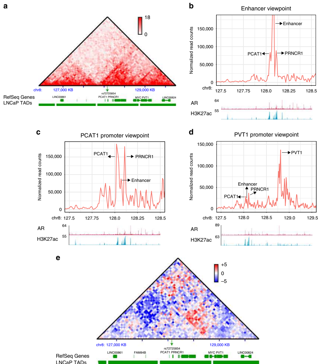
Fig. 3 The enhancer physically interacts with lncRNA promoters. a The TAD structure overlaid with gene annotations at the 8q24 region as seen from the HiC data in LNCaP cells. b Plots show 4C on the enhancer viewpoint using 4C-ker pipeline. c 4C plots from PCAT1 promoter viewpoint and d long-range interaction from 4C at PVT1 viewpoint, note the interactions marked by arrows. Tracks below the 4C plots in b-d show the ChIP-seq signal of AR and H3K27ac at the regions. e Comparative HiC in LNCaP and T47D showing the differential interactions at the 8q24 locus in the two cell lines. The red pixels show higher interactions in LNCaP and the blue ones show higher interactions in T47D, the heatmap is overlaid with gene annotations and TADs boundaries. 4C data are provided as source data file.
